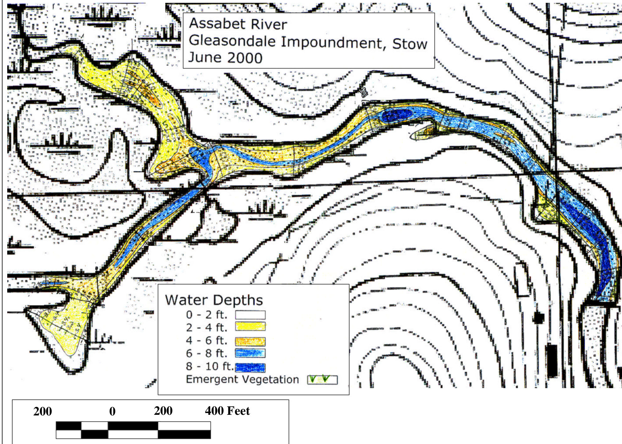
Figure 6-3 Assabet River: Bathymetry of Gleasondale Impoundment, Stow (RM 14)
